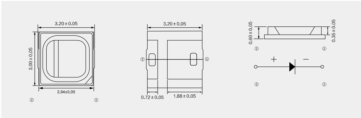
All dimensions are in millimeter)
